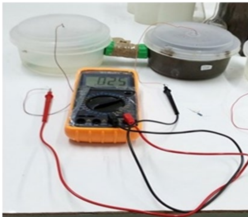
Figure 2.1: Set-up of H-shaped microbial fuel cells open circuit voltage
