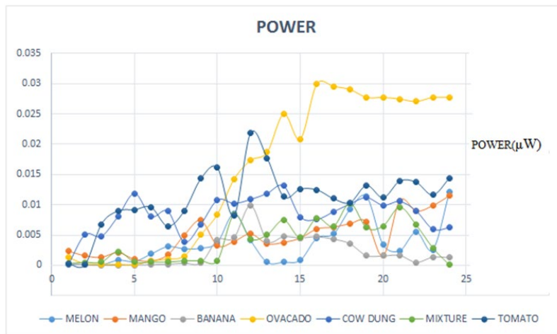
Figure 3.3: Plot of power against time generated by different fruits wastes.
