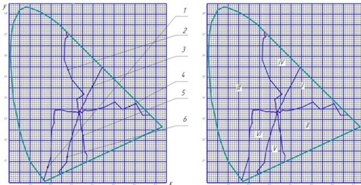
Figure 10 - The calibration curves in the XY plane
