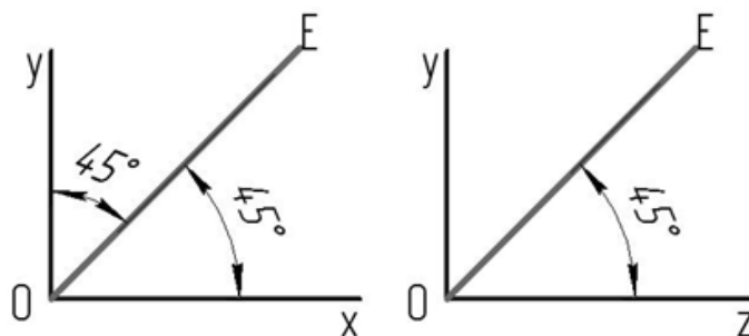
Figure 15 - Location OE vector with respect to space XYZ axes Vector OE will use the following way: it project the vectors of the two available samples and the resulting pre-registration and conversion device digital coordinates of the vector object (Figure 16).
