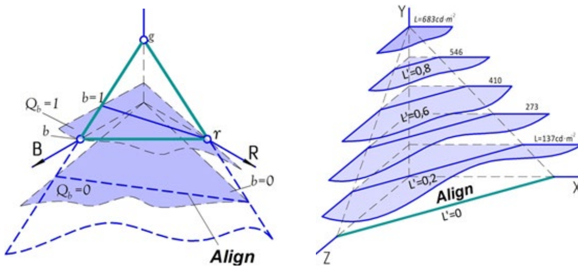
Figure 2- Planes and lines of equal brightness: a–in RGB-space;b– in XYZ-space
