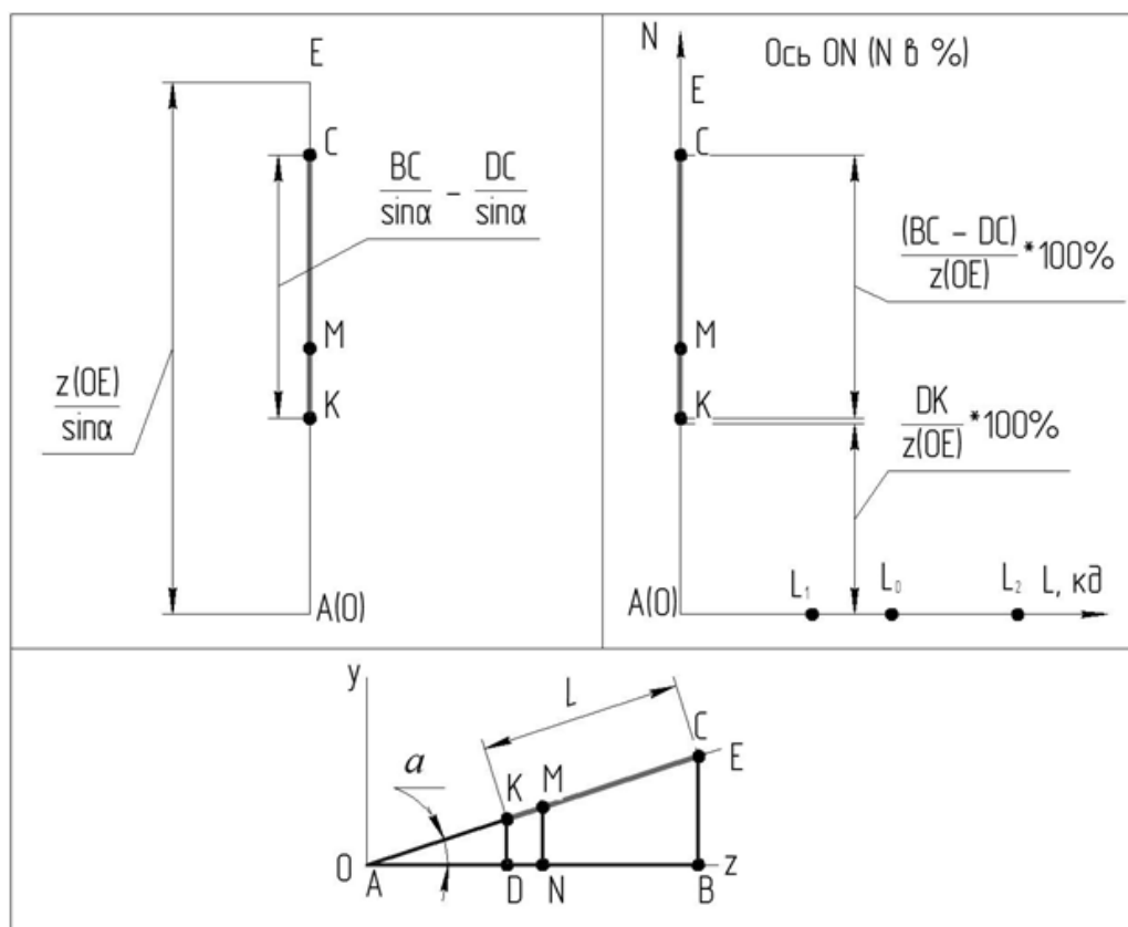
Figure 18 - Finding the size and location of the vectors point in the new coordinate system
