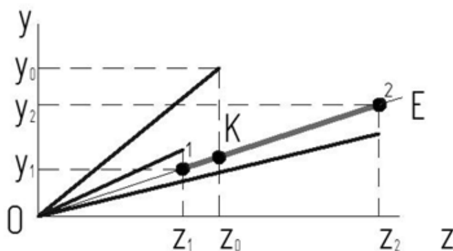
Figure 16 - The projections on the vector OE
