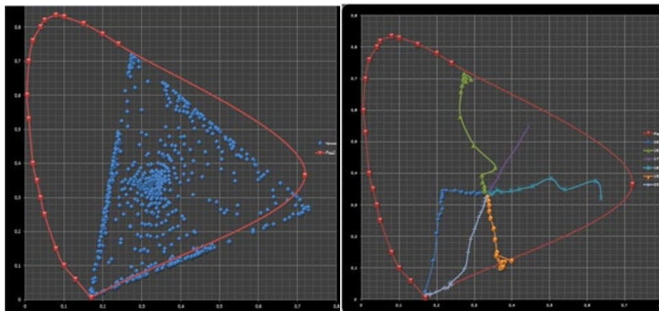
Figure8 - Projection vectors XYy (whole palette) Roman numerals from I to IV are indicated sectors corresponding to the sectors in Figure 9
