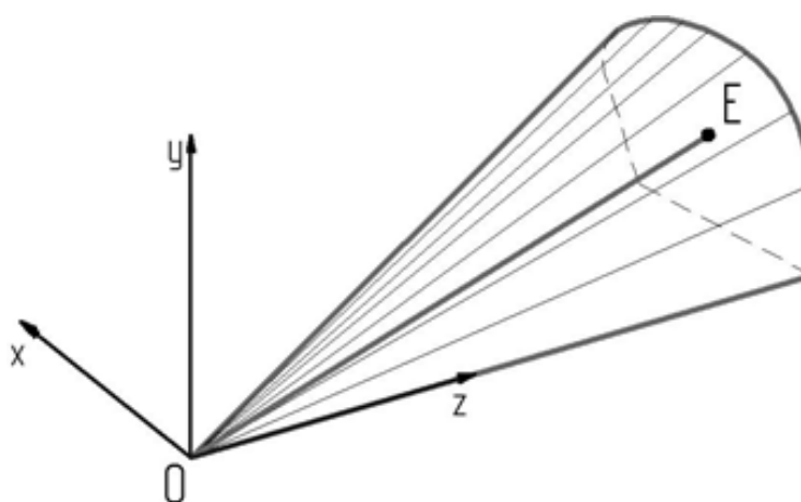
Figure 11 - Location in space XYZ direction vector to the white point
