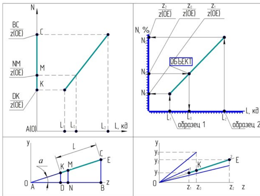
Figure 19 - Construction of the calibration straight line pattern
