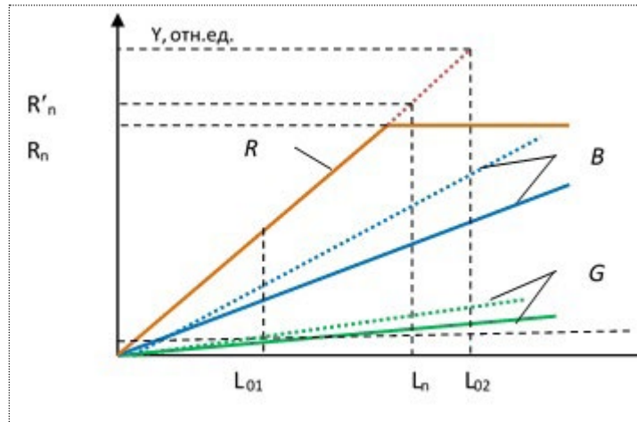
Figure 6 – The calibration curves of digital images color channels
